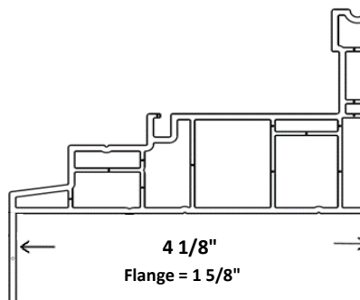
Tofino 8000 Series Casement/Awning- Reno/Rebate, Frame # 6301, Triple Pane Only
